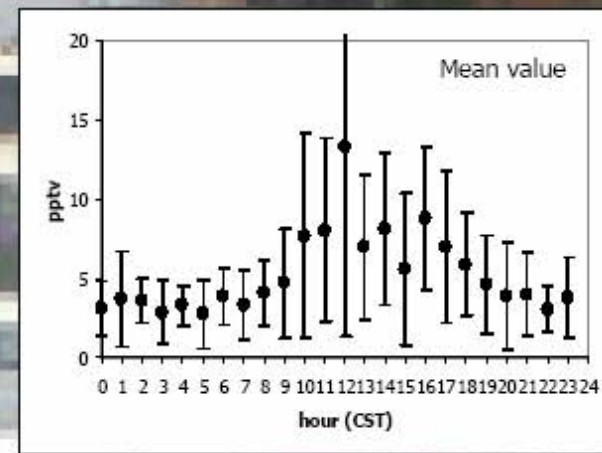
Figure 2: Daily Pattern of Maleate, the Potential Tri-carboxylic Acid with Base Peak m/z 87 and Oxalate in the Aerosol Phase
